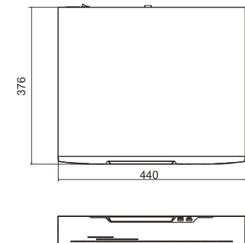
Figure 2-1 Dimensions (Unit:mm)
