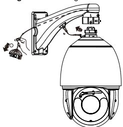
Figure 3-2 Fixing camera
