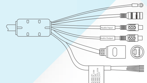
Figure 2-2 Multi-head cable
