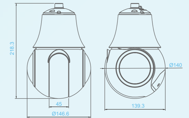
Figure 2-3 Dimensions(unit:mm)
