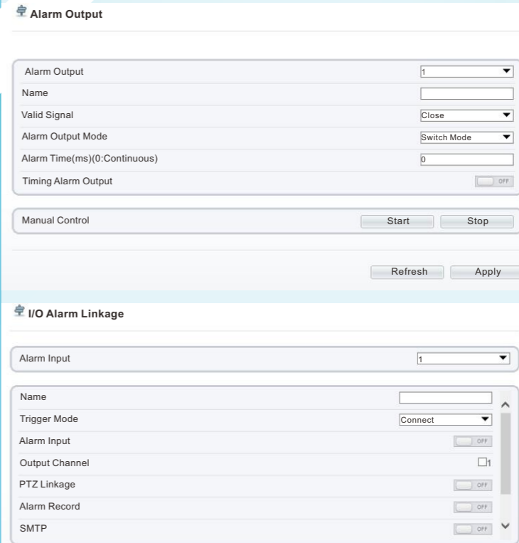
Figure 4-6 Alarm
