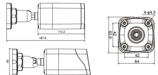
Figure 2-3 Dimensions (Unit: mm)
